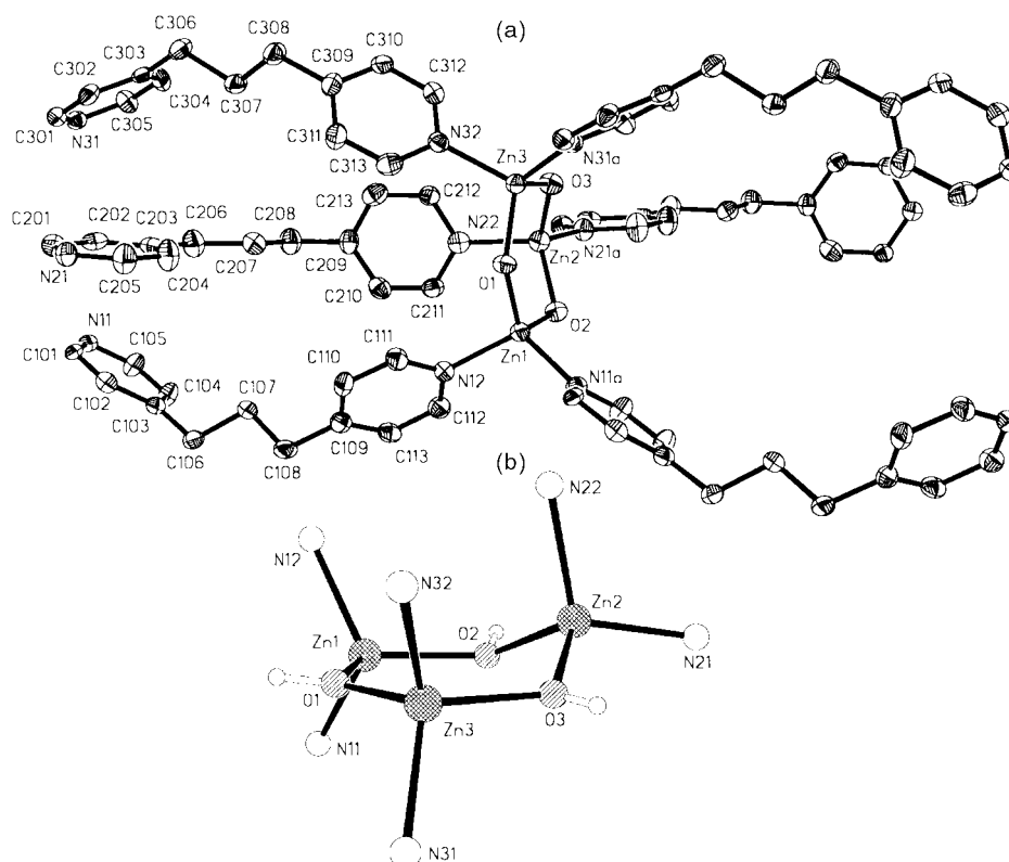
Fig. 1 Top: drawing of a building block for compound 1 showing the atom numbering scheme. Bottom: drawing of the \text{Zn}_3(\text{OH})_3 building block showing the puckered 6-membered ring. Selected dihedral angles for the ligand [ ^\circ ]: \text{C103-C106-C107-C108} -178.96 ; \text{C106-C107-C108-C109} -179.28 ; \text{C203-C206-C207-C208} 179.36 ; \text{C206-C207-C208-C209} -179.86 ; \text{C303-C306-C307-C308} -178.95 ; \text{C306-C307-C308-C309} -176.72 .
